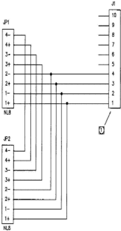
Connector Assembly 350991-001
