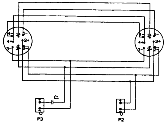
C1 Capacitor 39 uF / 160 VAC 963439
