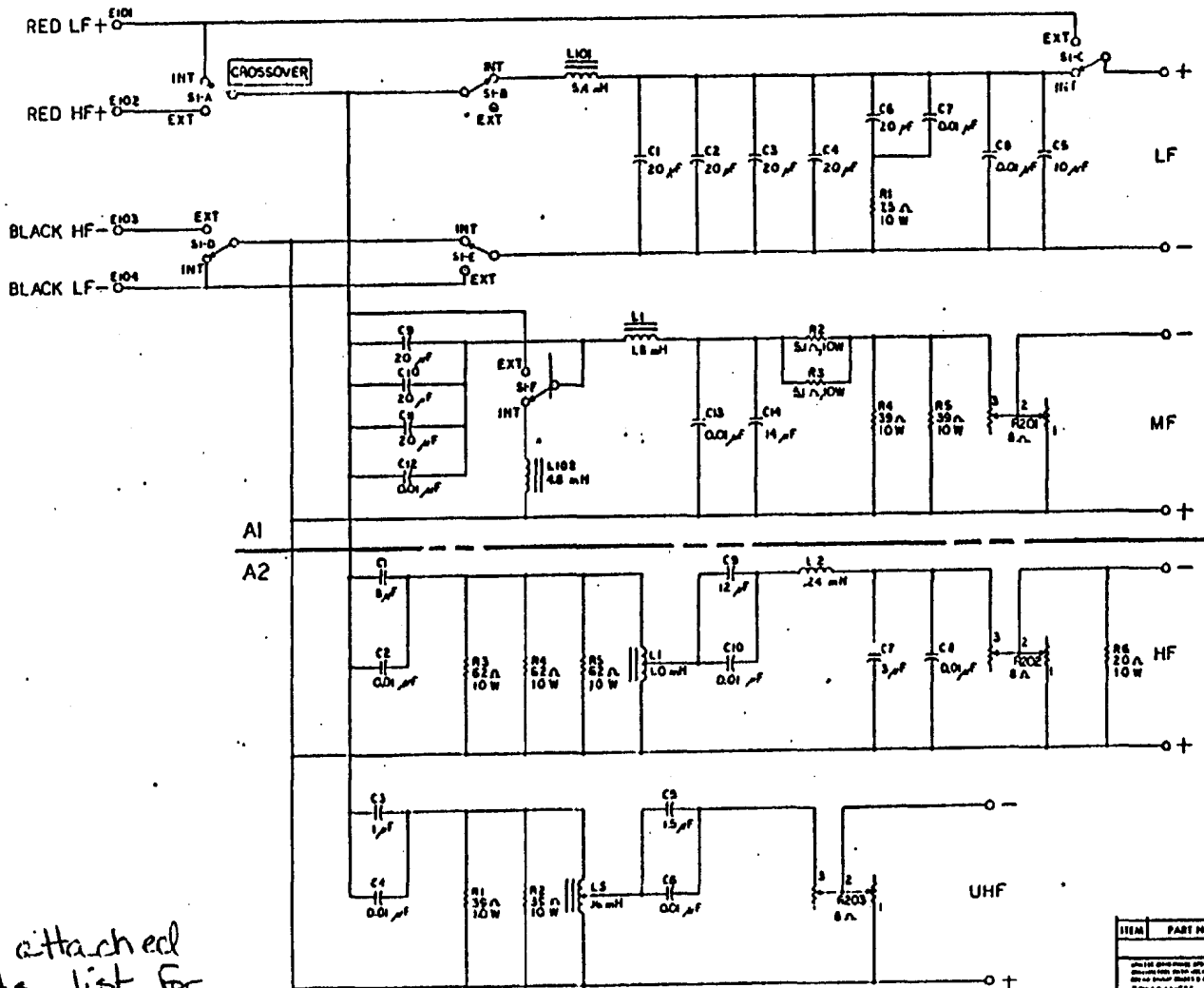
SIMPLIFIED SCHEMATIC
