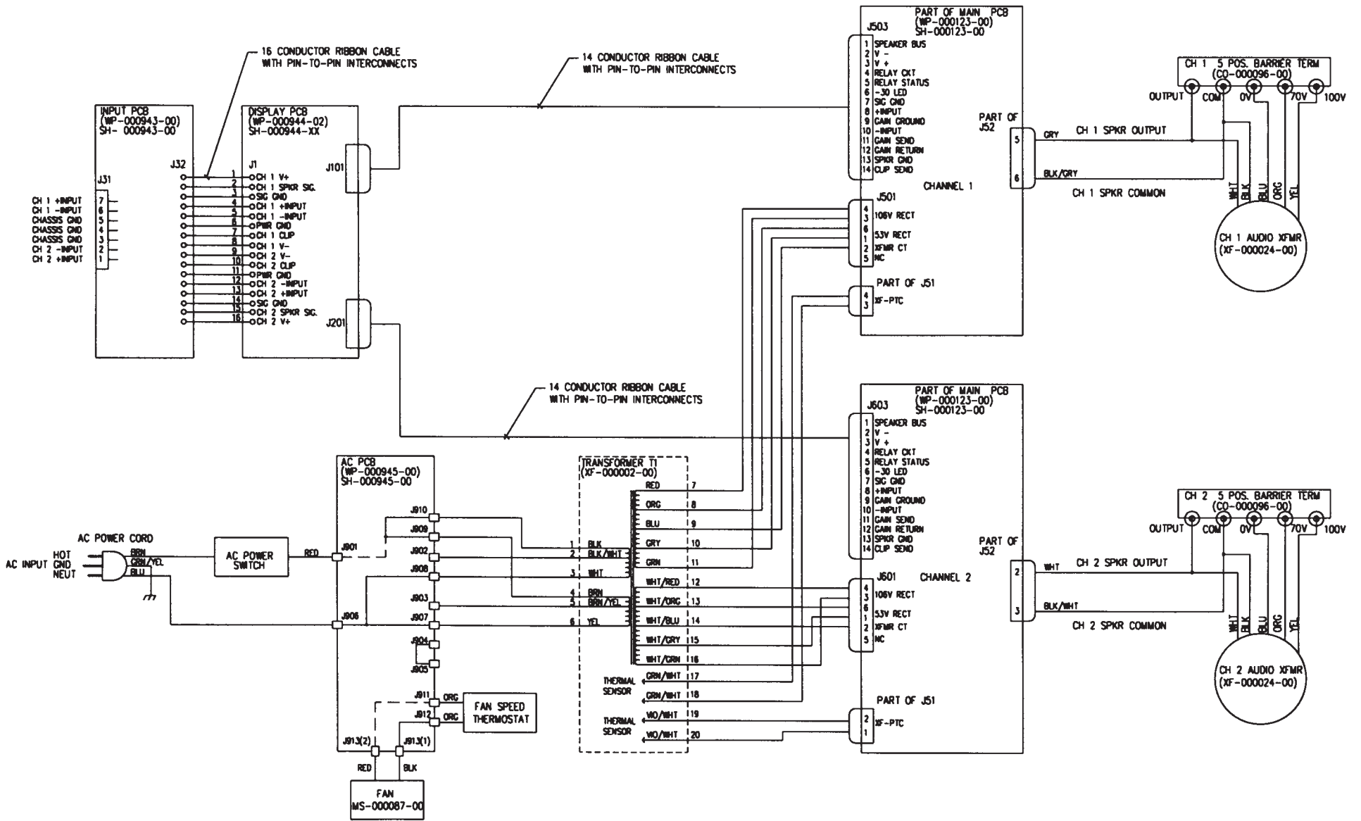
WIRING DIAGRAM, MPC600T
