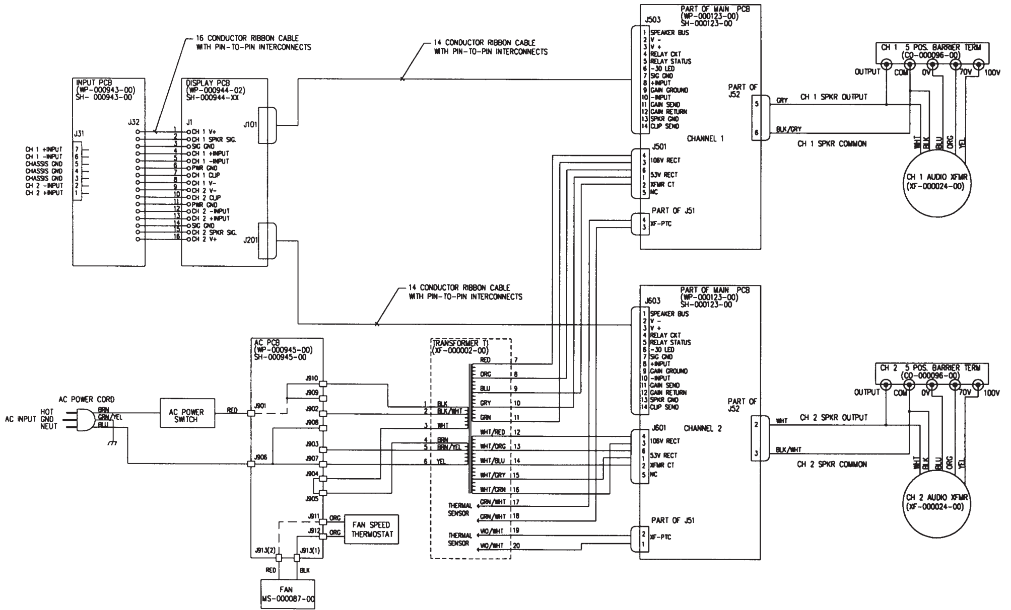
WIRING DIAGRAM - MPC600T, 230V SHOWN
