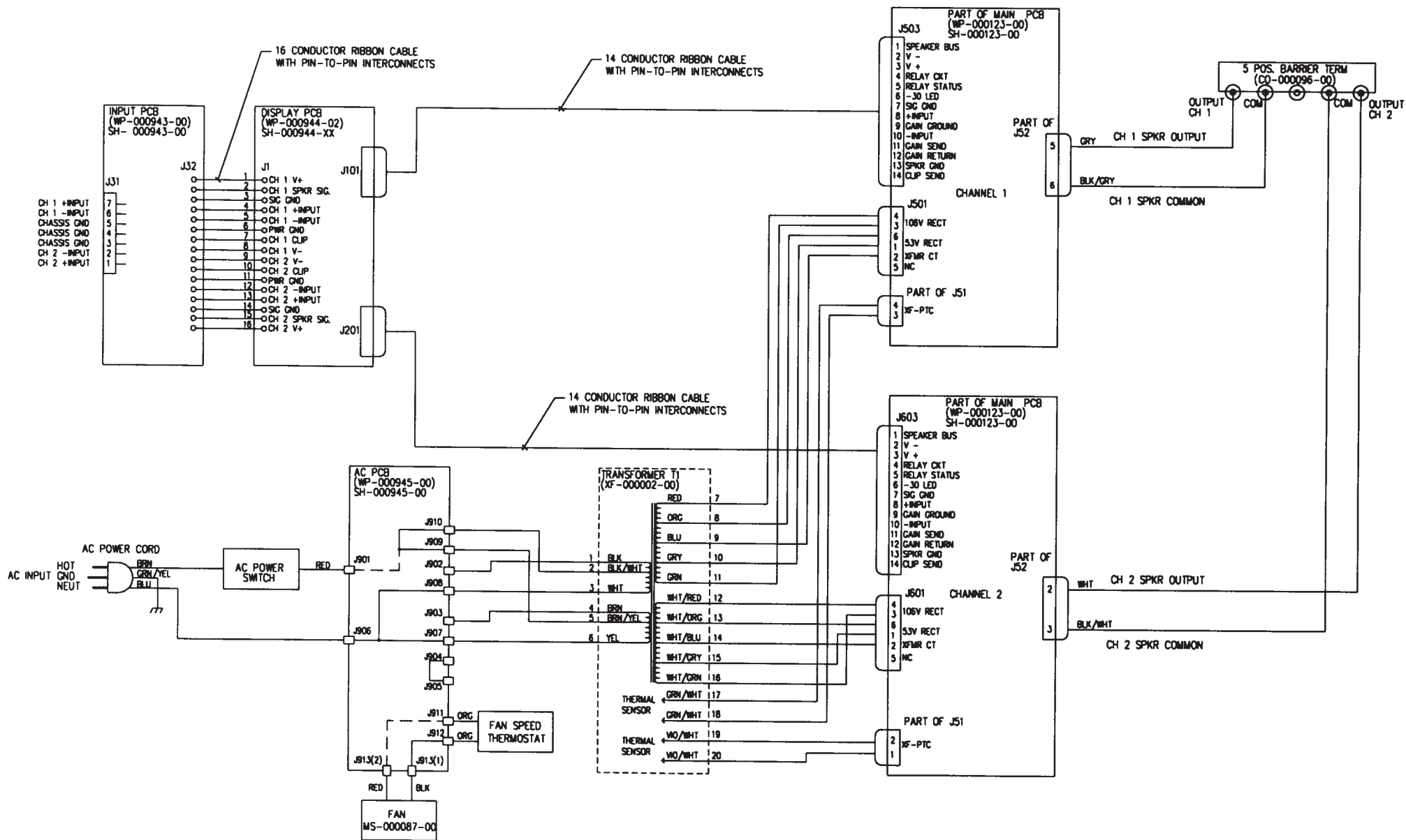
WIRING DIAGRAM - MPC600, 100V SHOWN
