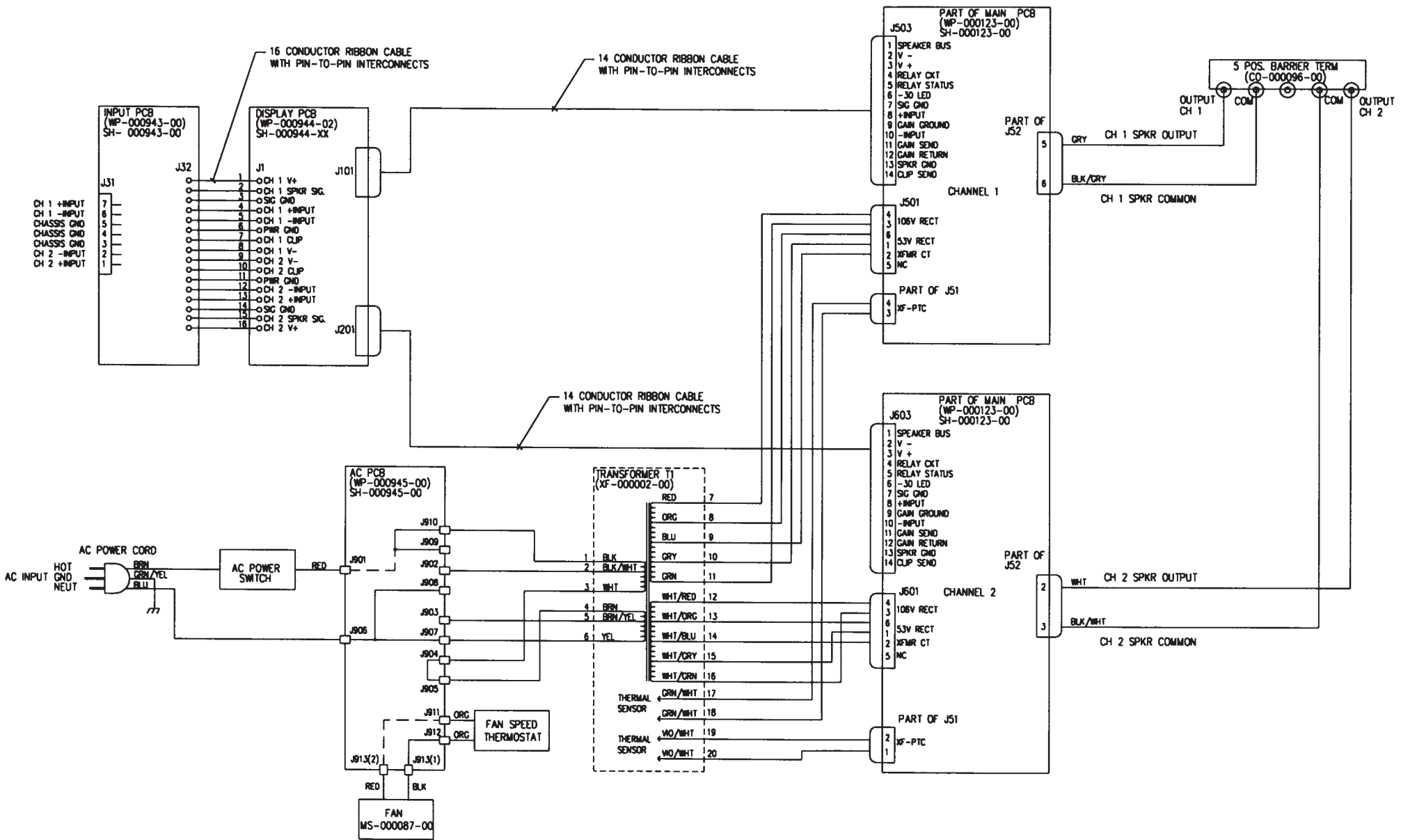
WIRING DIAGRAM - MPC600, 230V SHOWN
