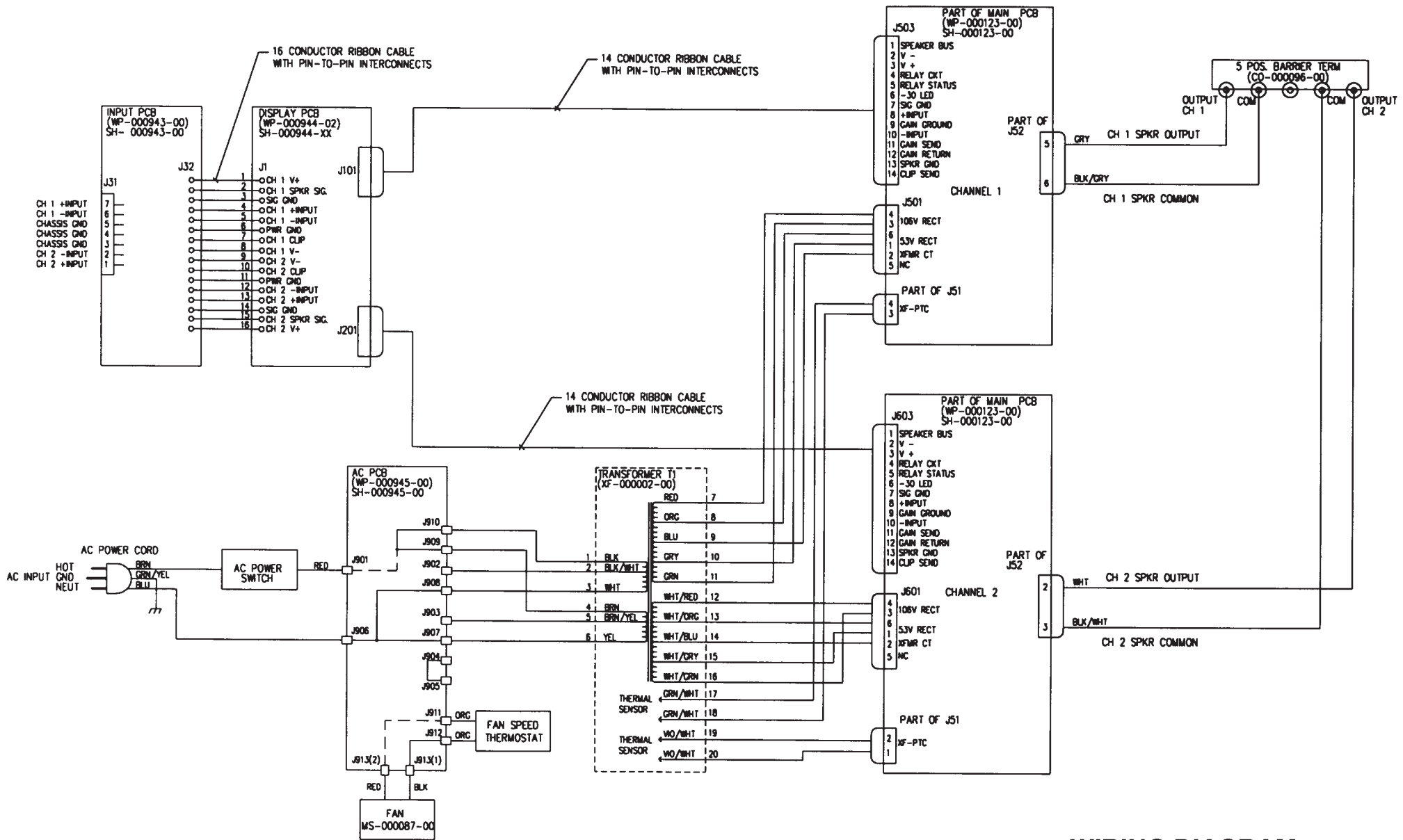
WIRING DIAGRAM, MPC600
