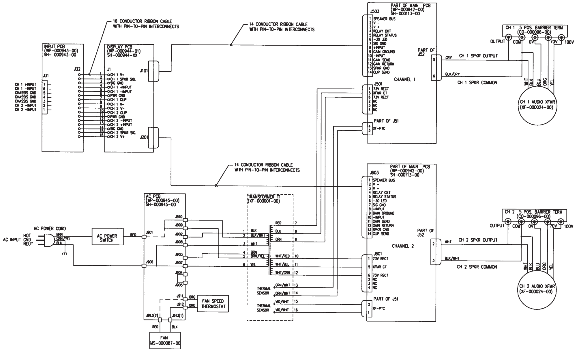
WIRING DIAGRAM - MPC300T, 100V SHOWN
