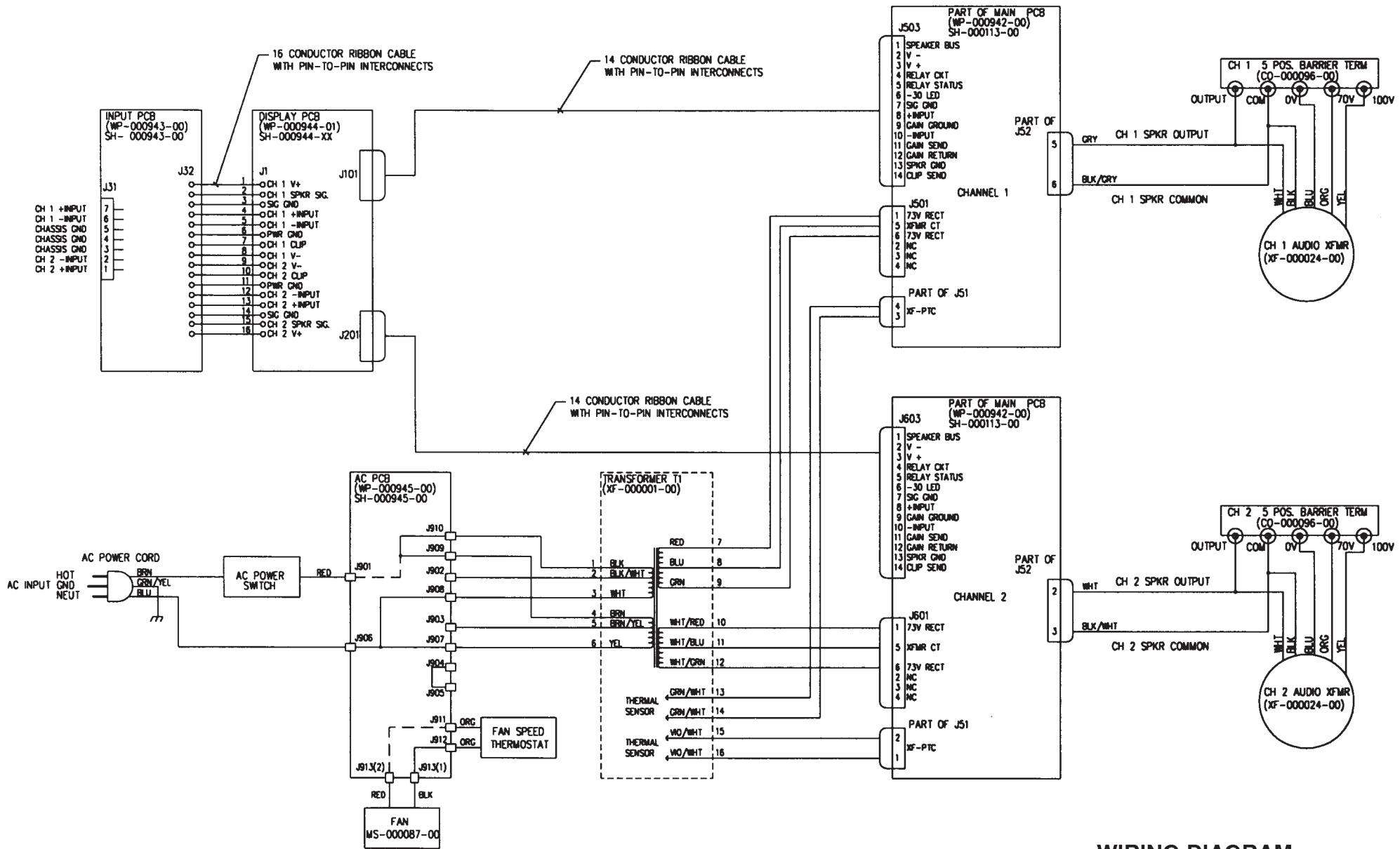
WIRING DIAGRAM, MPC300T
