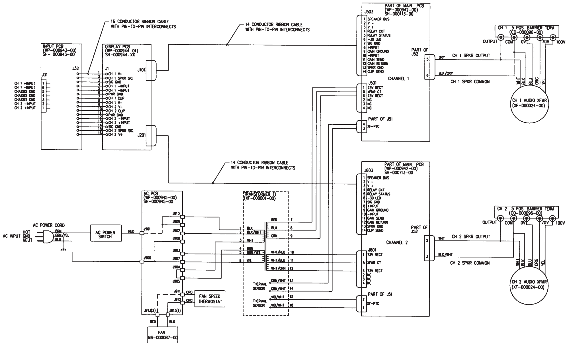
WIRING DIAGRAM - MPC300T, 230V SHOWN
