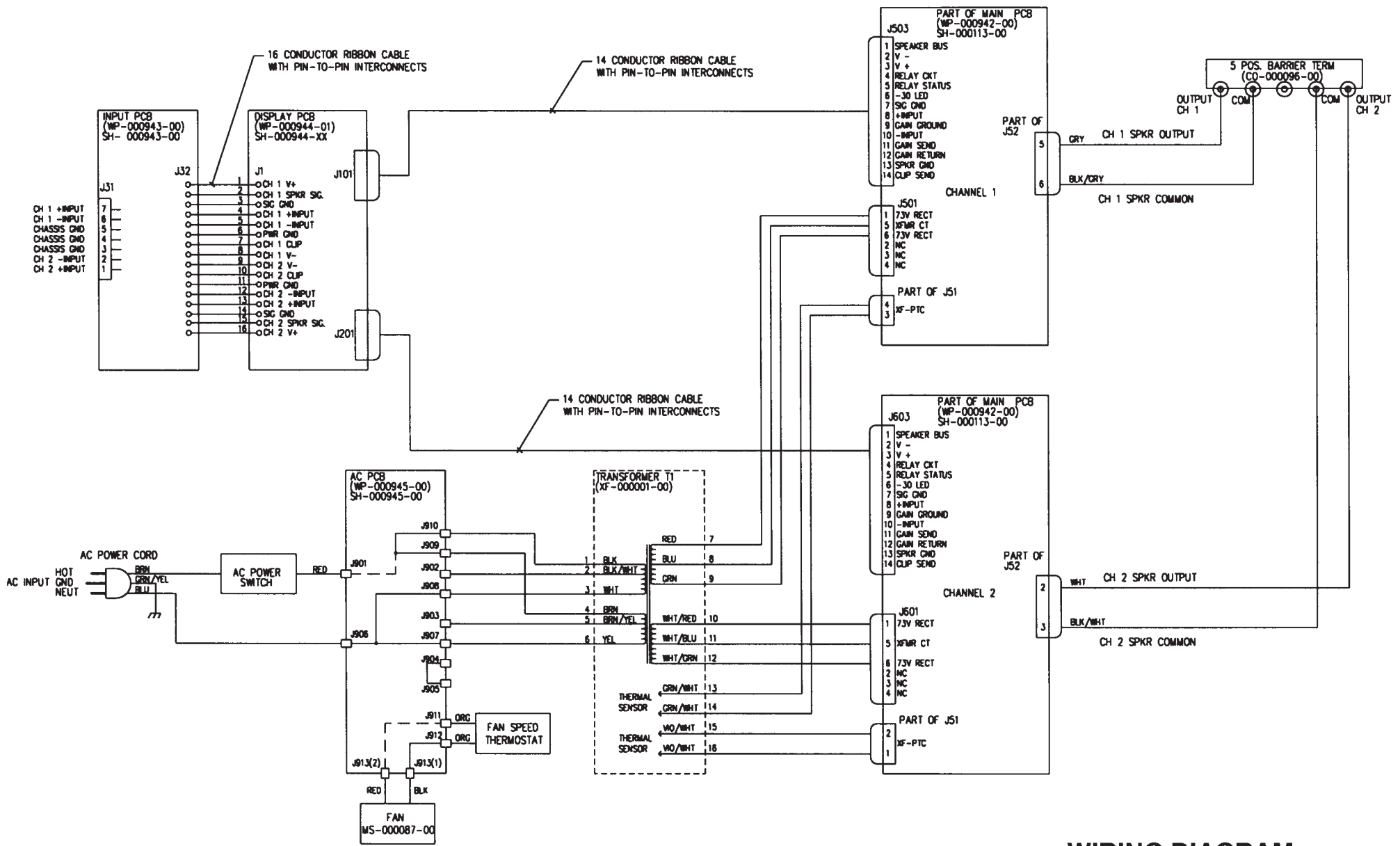
WIRING DIAGRAM, MPC300
