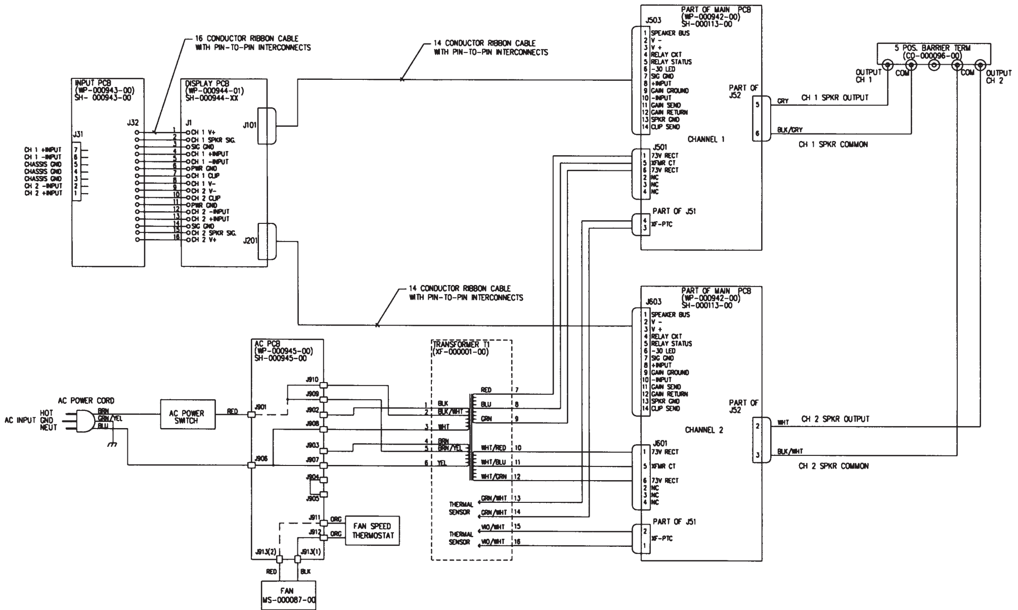
WIRING DIAGRAM - MPC300, 100V SHOWN
