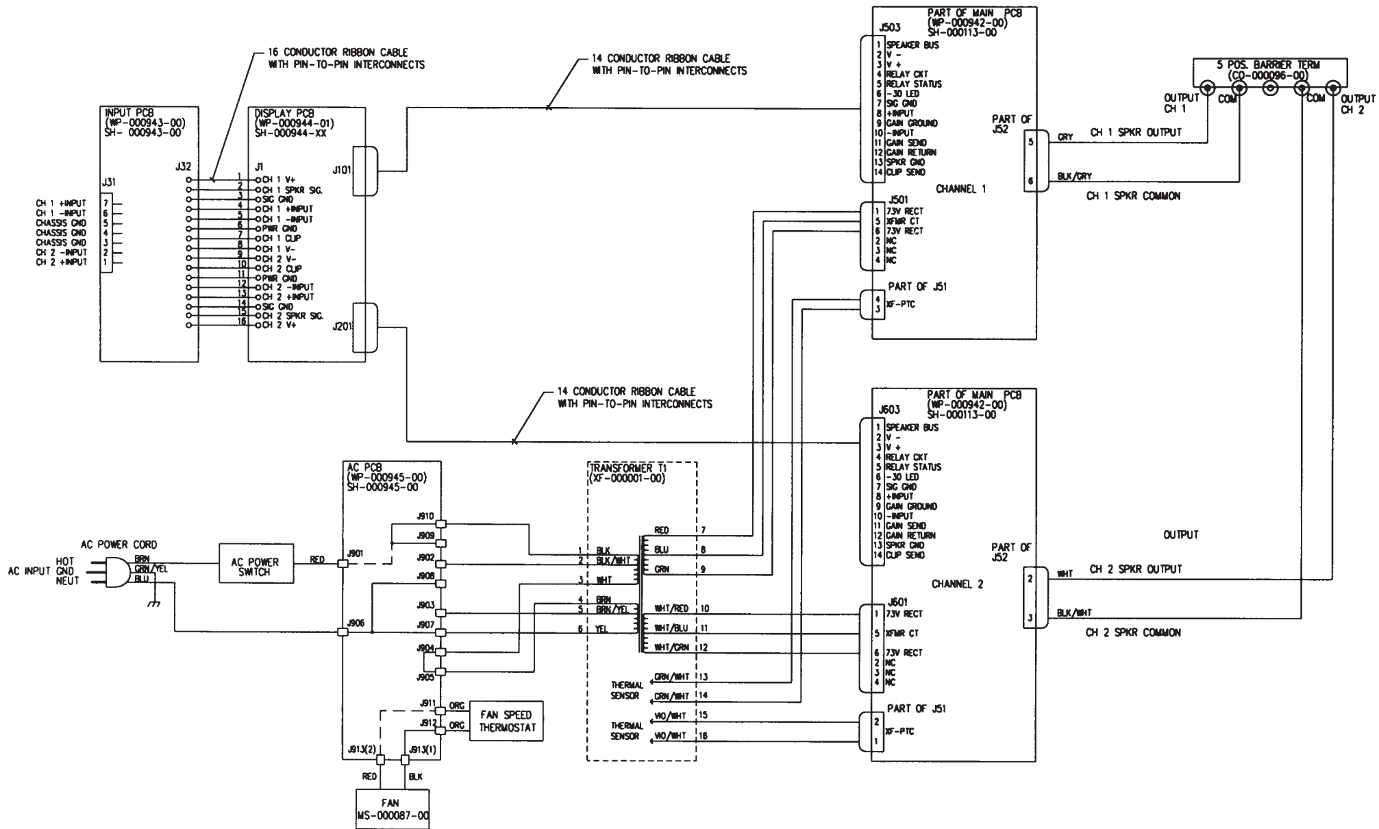
WIRING DIAGRAM - MPC300, 230V SHOWN
