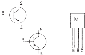
SMALL SIGNAL TRANSISTORS 2N4410 NPN / MPS8599 PNP
