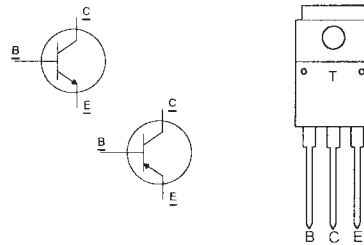
DRIVER TRANSISTORS 2SC3298 NPN / 2SA1306 PNP
