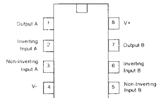
OP-AMP MC33178P Dual Operational Amplifier
