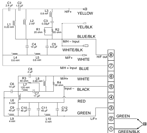
NETWORK SCHEMATIC: 350331-002
