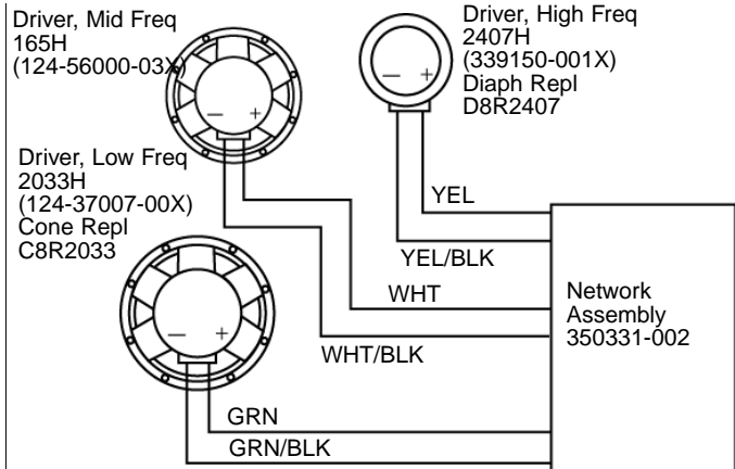
NETWORK SCHEMATIC: 350331-002
